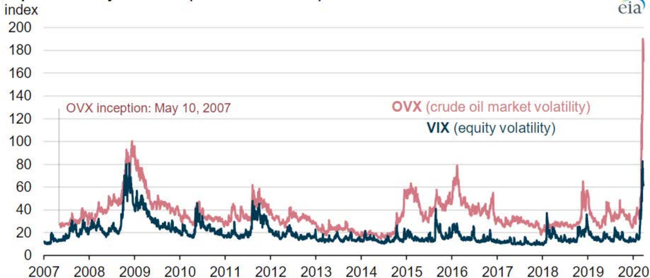
Implied volatility measures (Jan 2007-Mar 2020)
