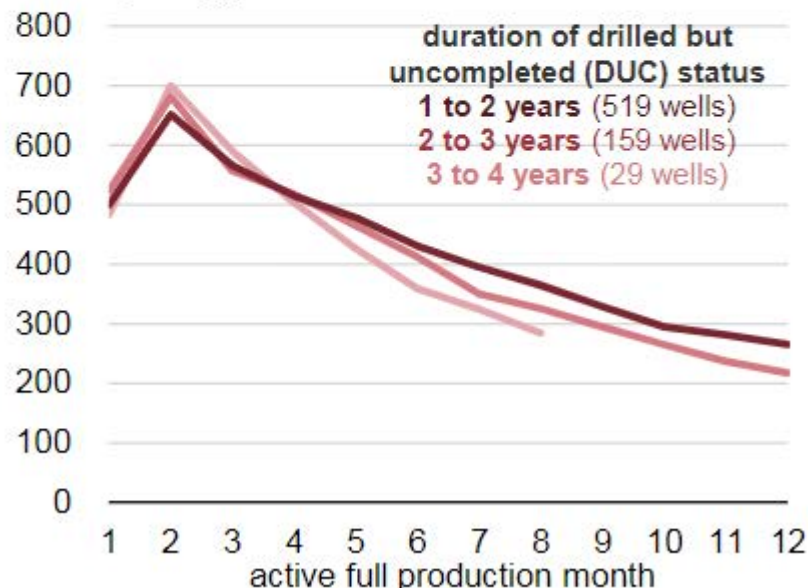
Average production from North Dakota crude oil wells initially drilled in 2014 through 2017
